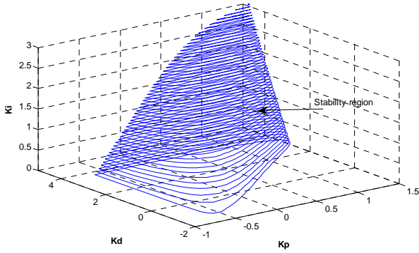
Figure 8: Stability region with PID Controller
