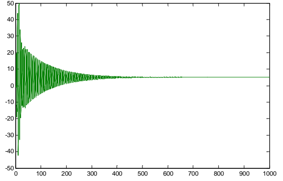
Figure 10: Closed loop step response with PID Controller ( K_p=0.6 , K_i=2.085 , K_d=4.2 ): stable case
