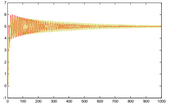
Figure 3: Closed loop step responses with PI Controller ( K_p=0.05 , K_i=0.1 : red response; K_p=0.1 , K_i=0.077 : green response): stable case
