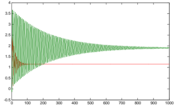
Figure 6: Closed loop step response with PD Controller (Kp=0.2, Kd=0.5: red response; Kp=0.41, Kd=0.5: green response): stable case
