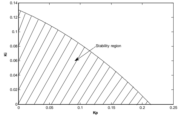
Figure 2: Stability region with PI Controller
