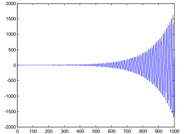
Figure 4: Closed loop step response with PI Controller ( K_p=0.2 , K_i=0.04 ): unstable case
