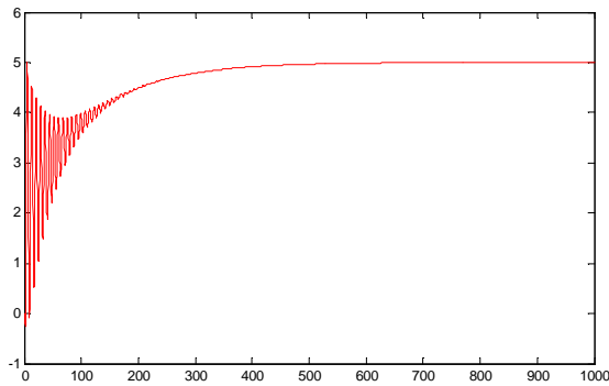
Figure 9: Closed loop step response with PID Controller ( K_p=1 , K_i=2.085 , K_d=4.2 ): stable case
